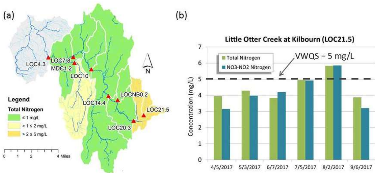
Figure 7. Nitrogen monitoring results for Little Otter Creek focus stations during 2017 including: (a) mean total nitrogen (TN) by water-quality subwatershed and (b) NO 3 -NO 2 and TN by sample date for station LOC21.5, relative to the Vermont Water Quality Standard of 5 mg/L for nitrogen as nitrate.
