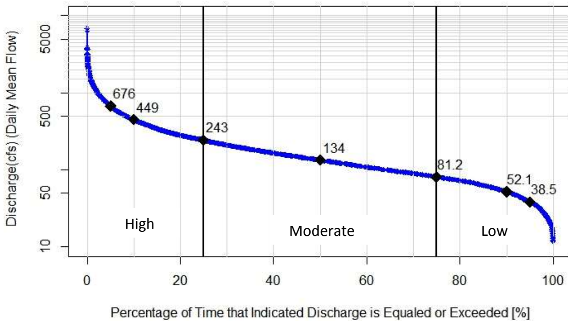
Flow Duration Curve for New Haven River @ Brooksville, wy1991-2016
