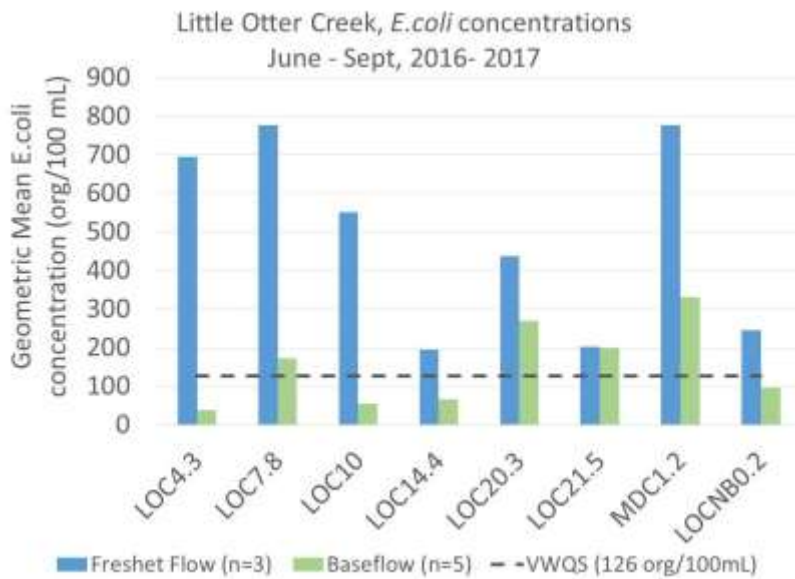
Figure 2. Geometric mean of E. coli monitoring results for Little Otter Creek focus stations during wet-weather, freshet flow events (in blue) versus dry-weather, baseflow events (in green) during focus monitoring years 2016 and 2017.
