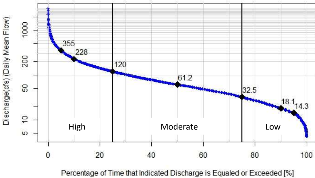
Flow Duration Curve for Lewis Creek @ N. Ferrisburg, wy1991-2016
