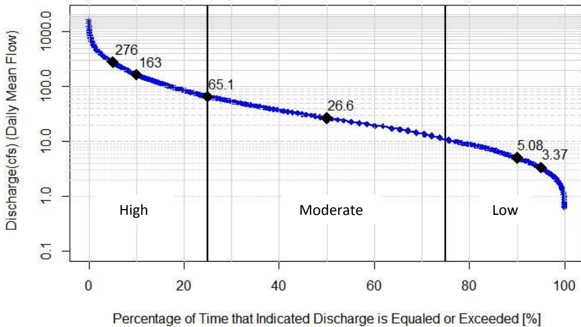
Flow Duration Curve for Little Otter Creek @ Ferrisburg, wy1991-2016
